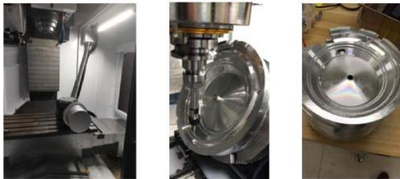
振动盘加工 (850+YHM200五轴转台) Vibration plate processing (850+YHM200 five-axis turntable)
